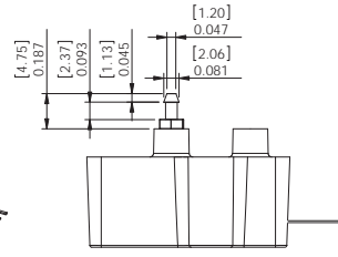
C- Barb Fitting Port B Only Configuration
